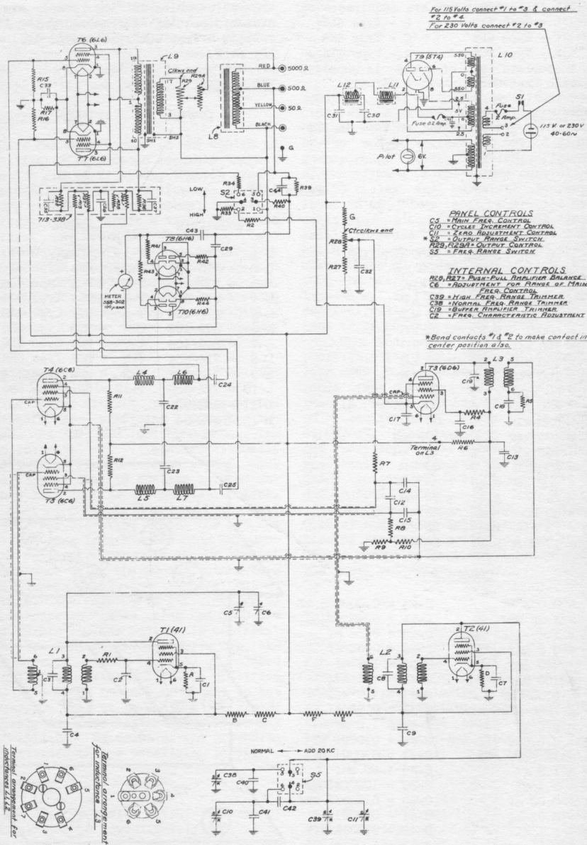
FIGURE 3. Wiring Diagram for Type 713-B Beat-Frequency Oscillator
